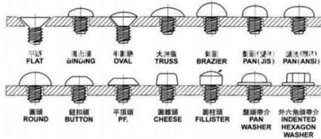
SCREW HEAD STYLES (頭型對照表)
