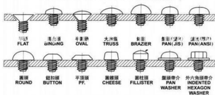
SCREW HEAD STYLES (頭型對照表)
